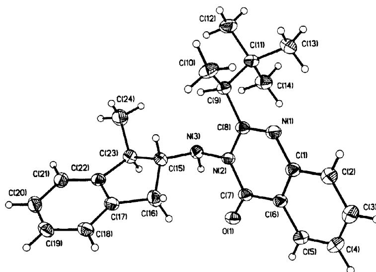
Fig. 1. ORTEP view of 12 (thermal ellipsoids are drawn at 50% probability level)
